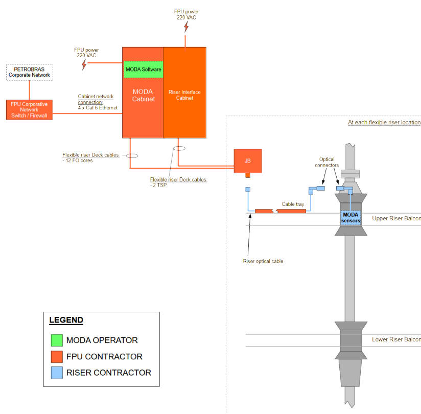
Figure 7: General Scopes at FPU.
