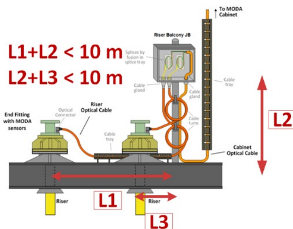
Figure 7: Riser JB distance requirement.
