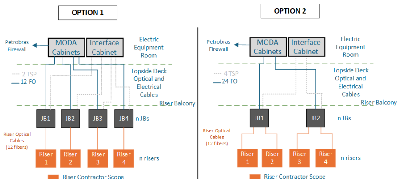
Figure 6: MODA recommended layout options.
