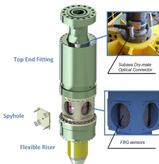
Figure 1: Spyhole End Fitting with MODA sensors.
